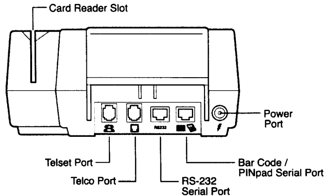
Figure 6 OMNI 3200 Connection Ports
