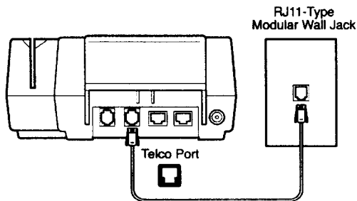
Figure 8 Direct Telephone Line Connection
